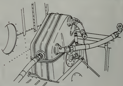
FIGURE 6-14. Disconnecting oil lines.
